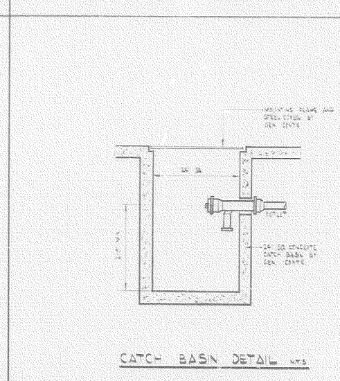
DETAIL OF STANDARD CATCH BASIN NTS
