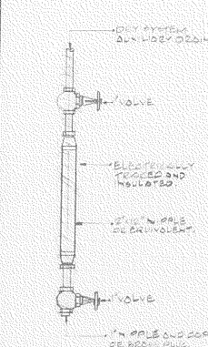
DETAIL OF DRAIN TRAP NTS
